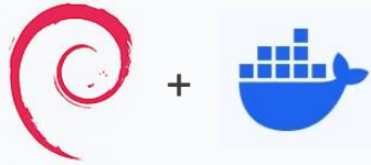
Debian Server
